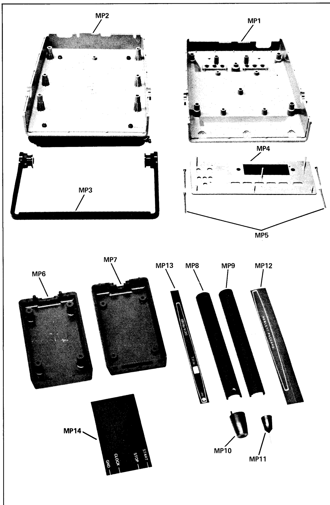
Figure 6-1. Mechanical Parts
